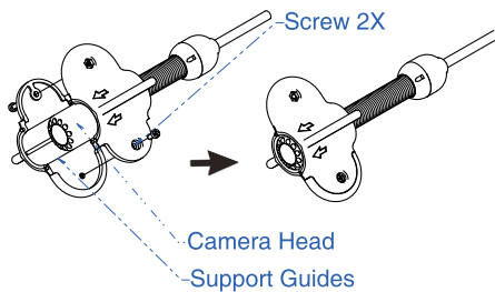
D80 Applicable to 3.5"-5" pipe. Figure 12. Install Support Guides
