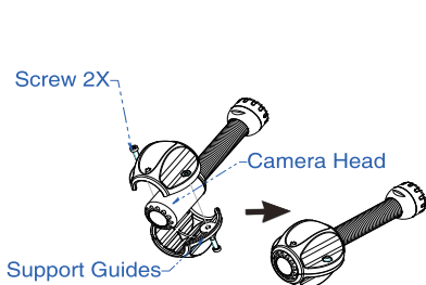
D46 Applicable to 2"-3.5" pipe. Figure 11. Install Support Guides
