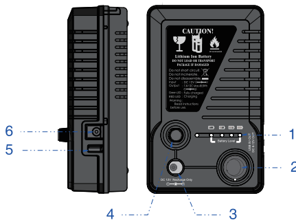
Figure 4. Battery pack
