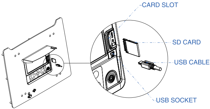
Figure 13. Install SD Card
